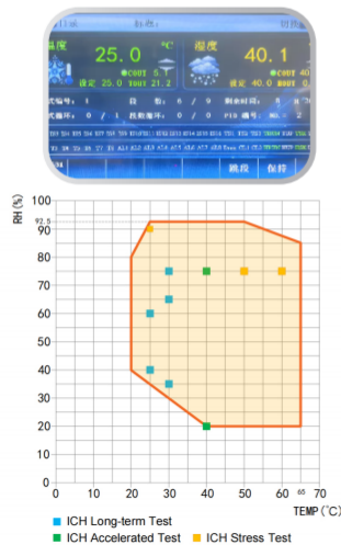
◆ 温湿度控制范围图 / Temperature and Humidity Control Range Diagram
