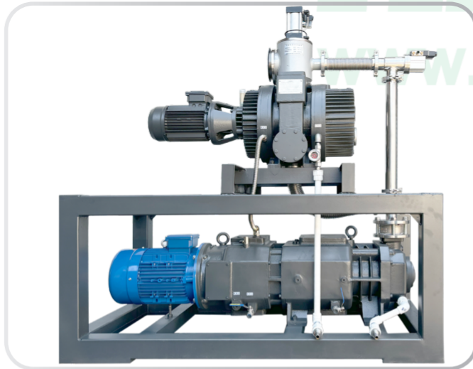
干式螺杆罗茨泵真空机组 Dry Screw-Roots Pumps Vacuum System
